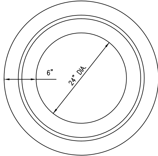
Plan (Jointed)
