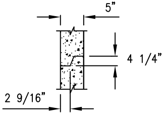
Joint Detail
