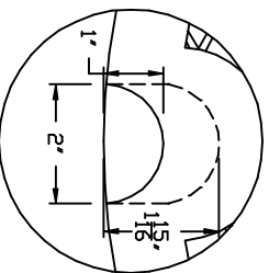
NON-PENETRATING PICKHOLE DETAIL
