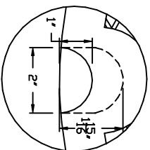
NON-PENETRATING PICKHOLE DETAIL
